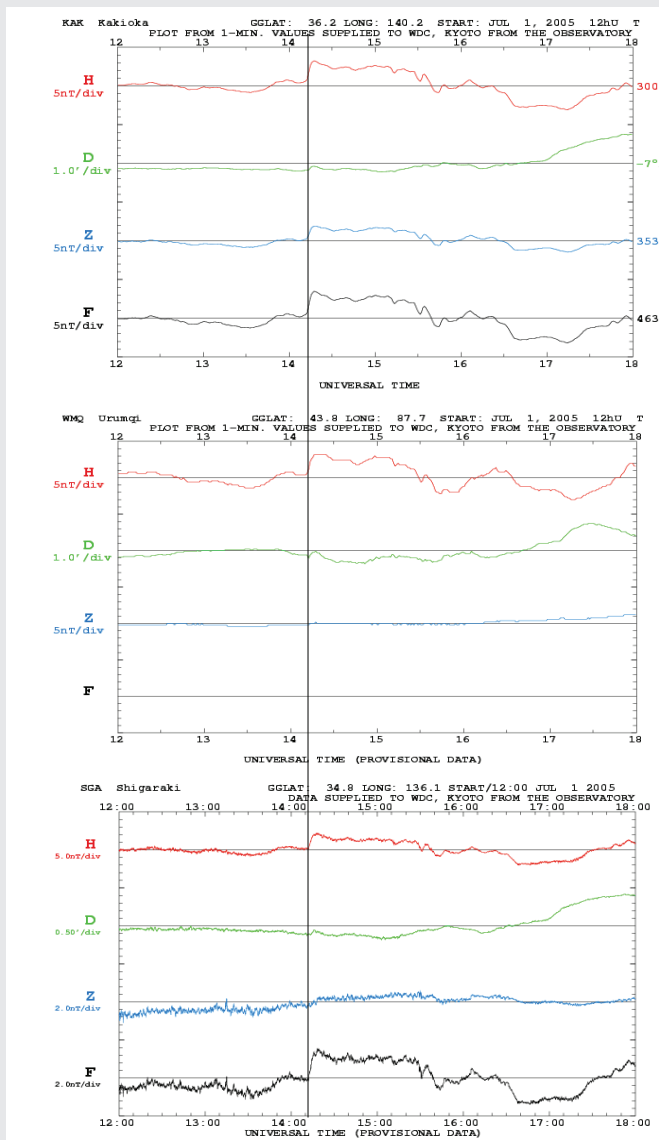
Figure 6: Magnetometer responses to the arrival of the co-rotating interaction region at the magnetopause on July 1 st , at Kakioka, Urumqi, and Shigaraki. The vertical line marks the sudden commencement at 14:12 UT.
