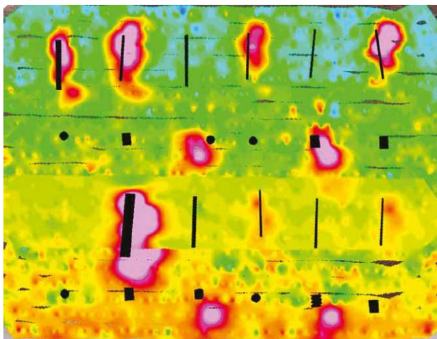
FIGURE 26. Geometric measurement of MF of the objects depicted in Fig 24) using the metal detector a .
