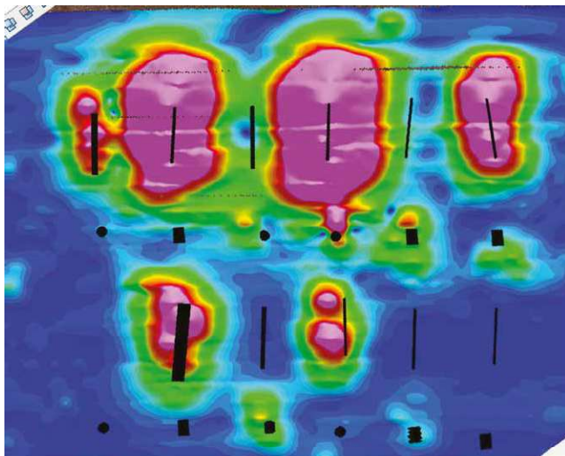
FIGURE 25. Geometric measurement of MF of the objects depicted in Fig 24) using the MagArrow Magnetometer a .
