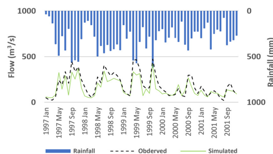
Fig. 4(b) Monthly hydrograph for validation (1997-2000) at Patupaula station from the HEC-HMS model.
