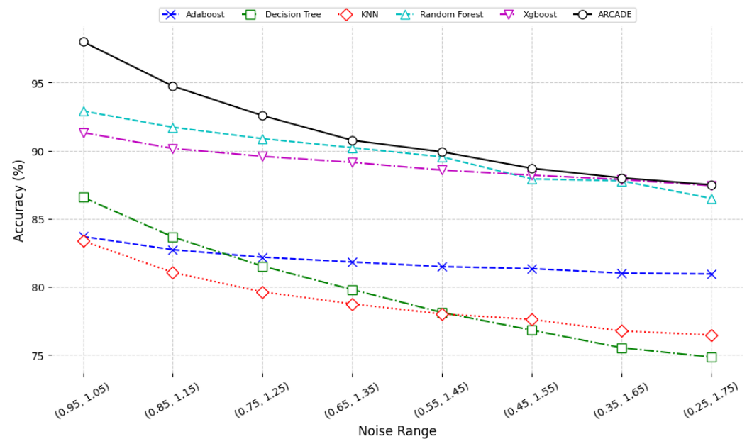
Figure 10. Performance comparison across range of adversarial attacks with four features altered.
