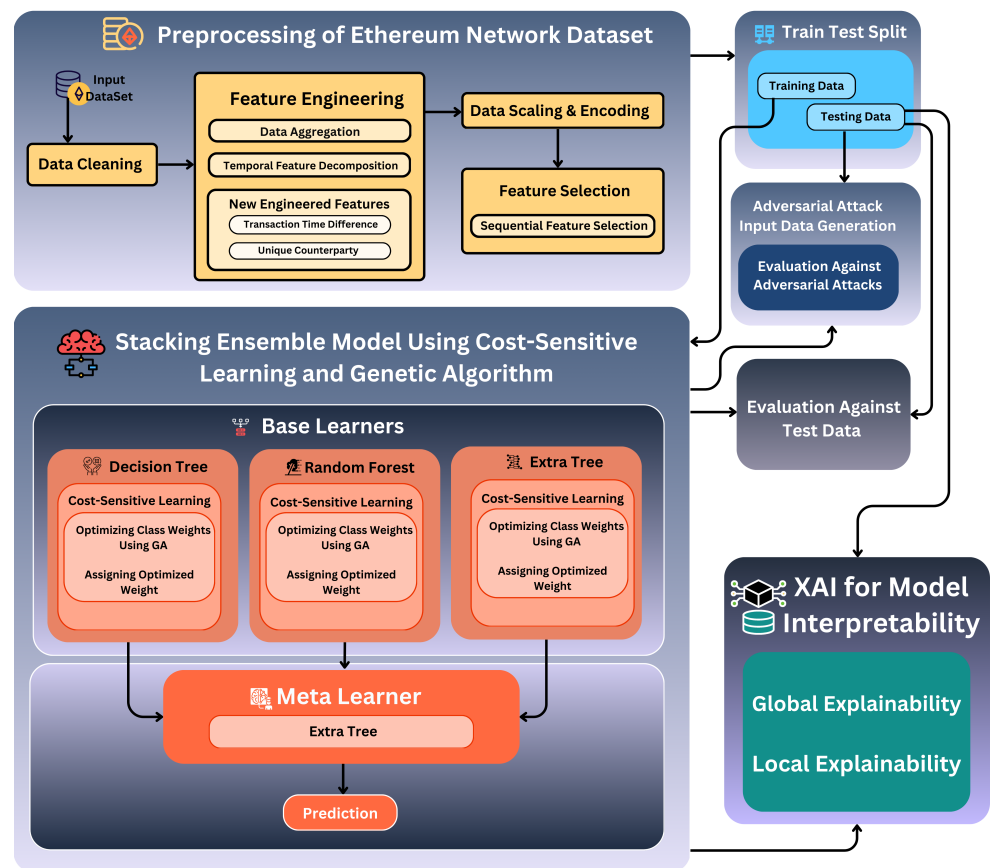
Figure 1. Proposed ARCADE methodology.
