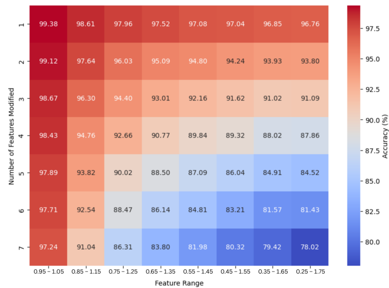
Figure 5. Accuracy: impact of feature range and number of features modified.
