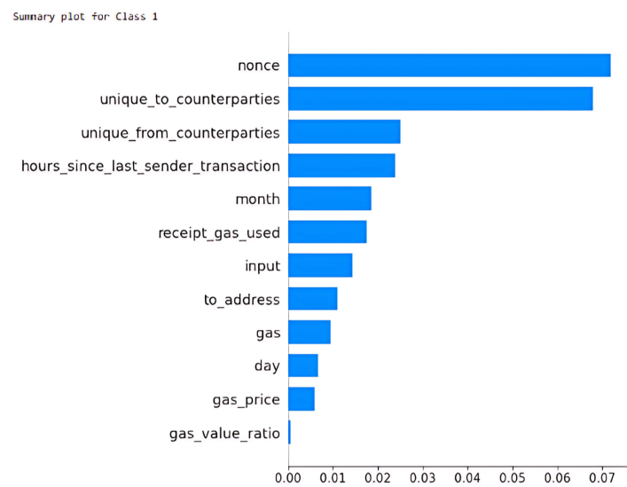
Figure 13. Global interpretation for Class 1.
