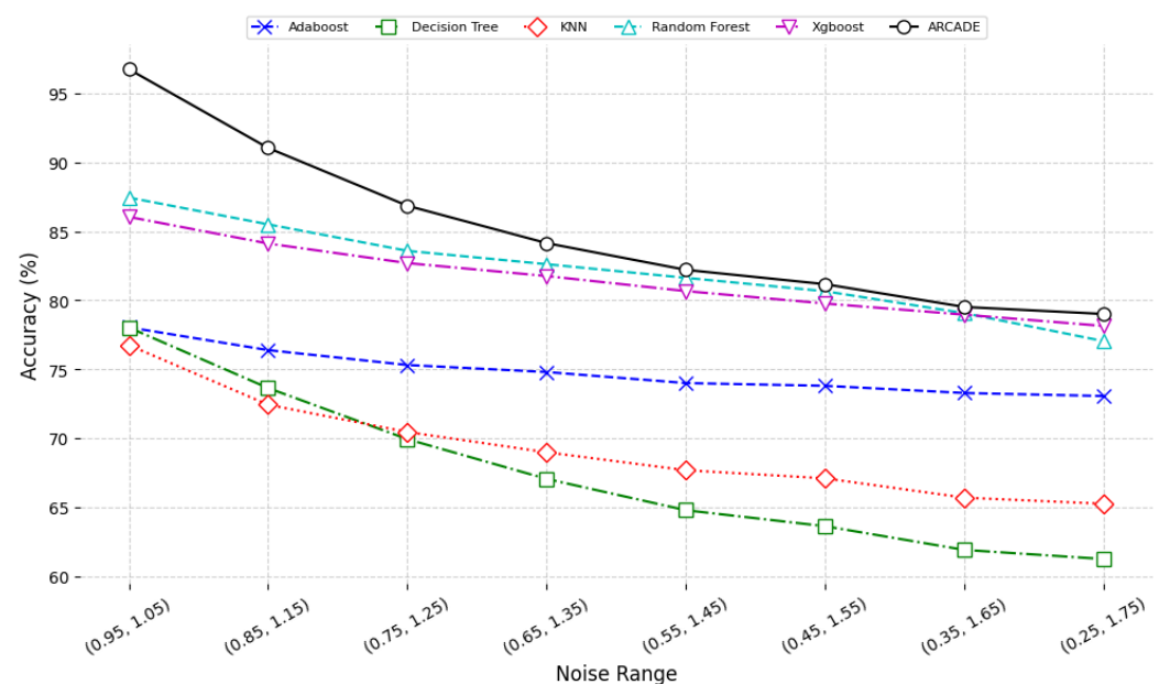
Figure 11. Performance comparison across range of adversarial attacks with seven features altered.
