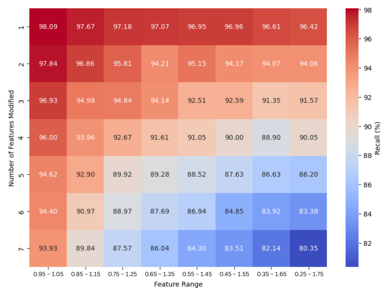
Figure 7. Recall: impact of feature range and number of features modified.
