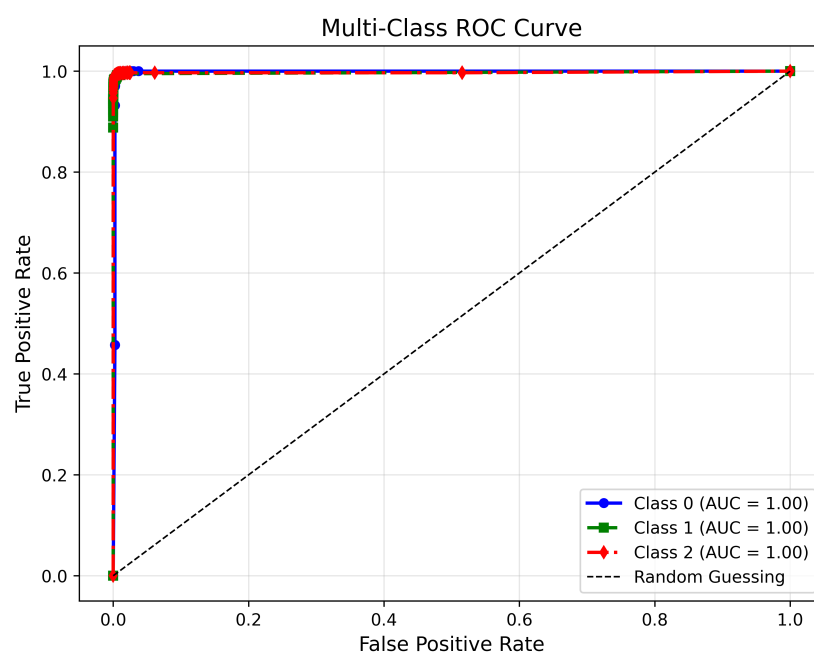
Figure 3. Multi-class ROC curve For ARCADE.
