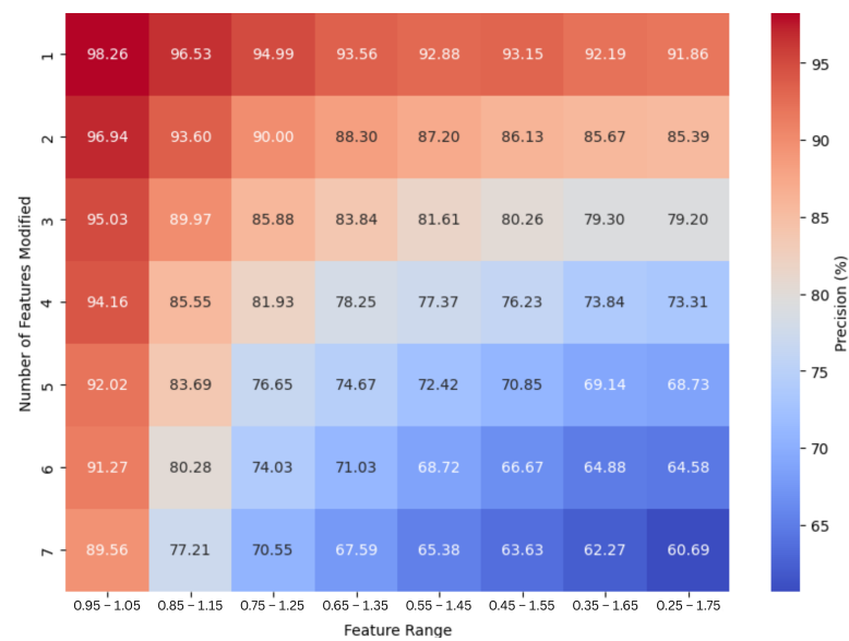
Figure 6. Precision: impact of feature range and number of features modified.
