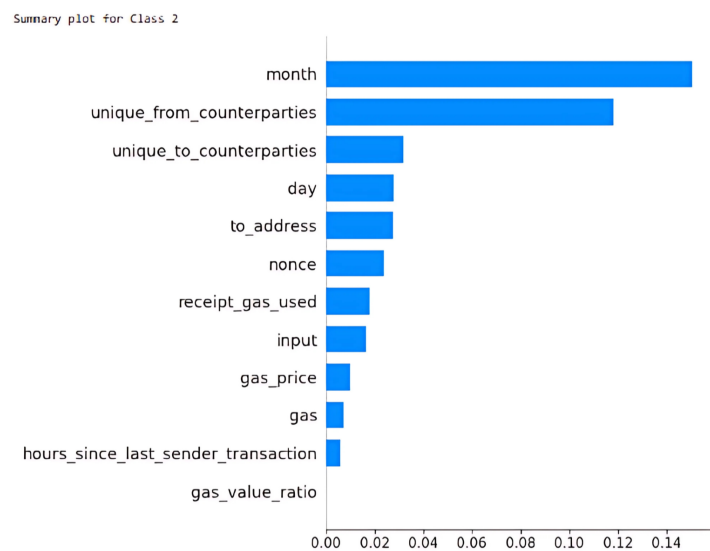
Figure 14. Global interpretation for Class 2.
