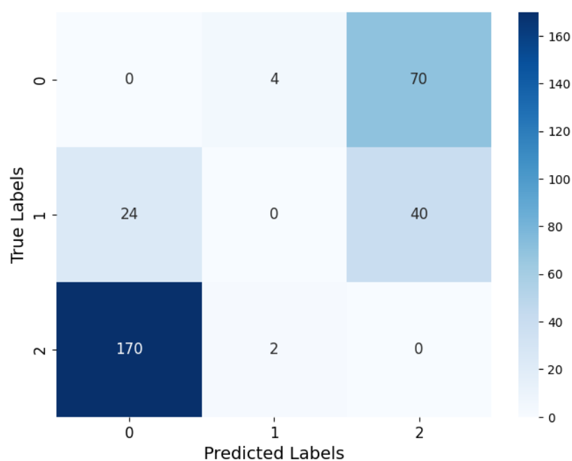
Figure 4. Cost-annotated confusion matrix.
