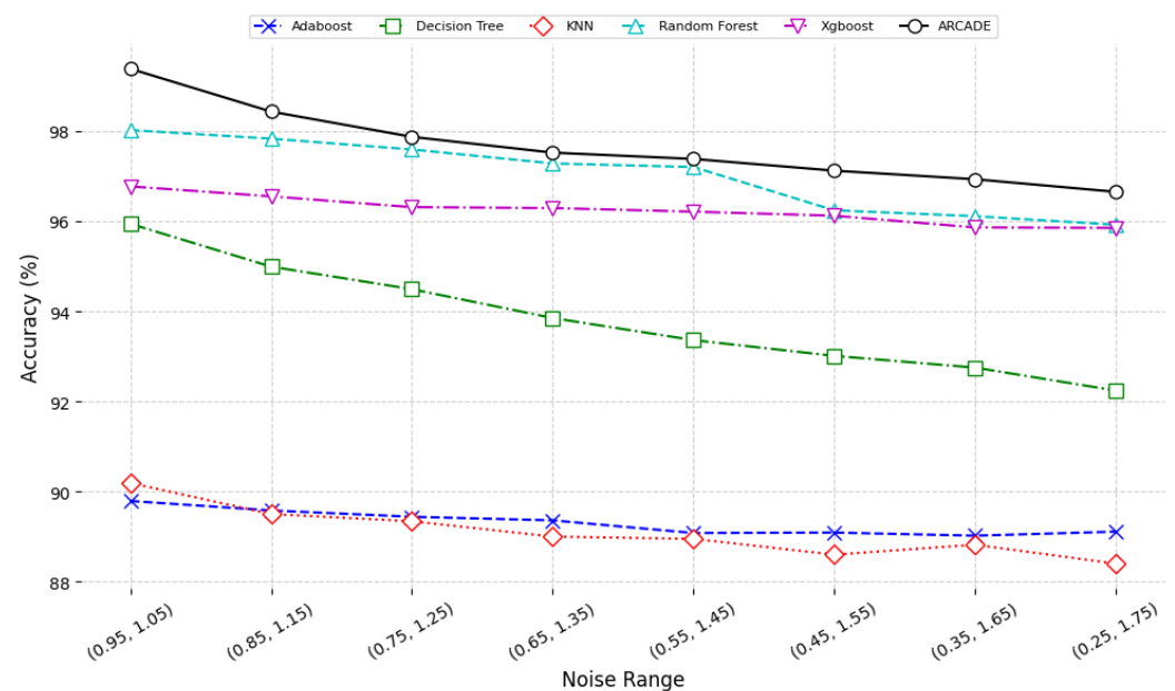
Figure 9. Performance comparison across range of adversarial attacks with one feature altered.
