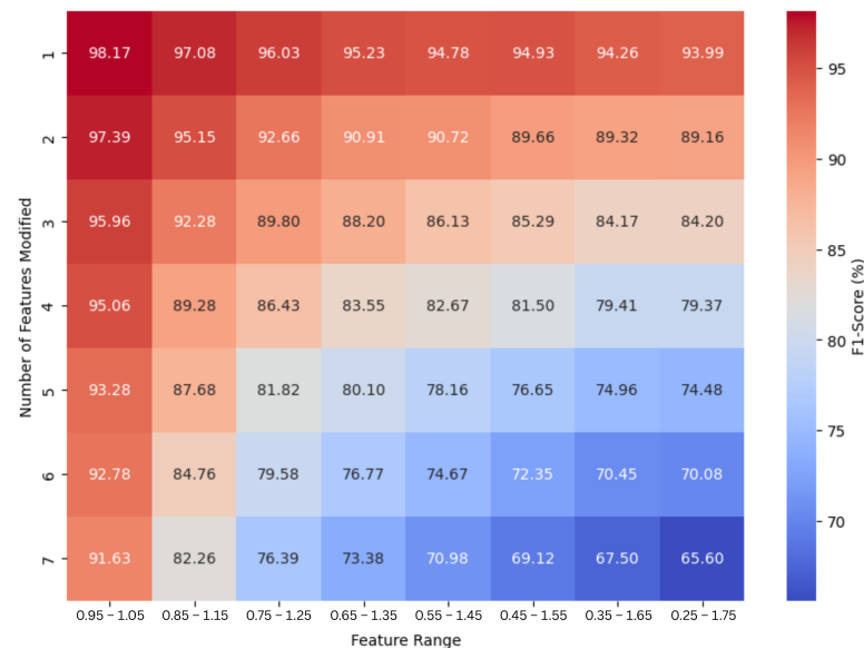
Figure 8. F1 Score: impact of feature range and number of features modified.
