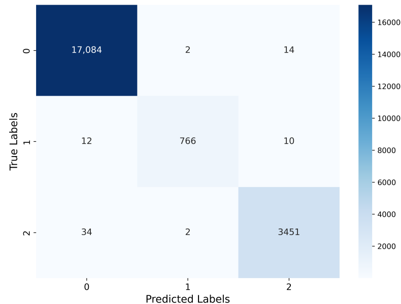
Figure 2. Confusion matrix for cross-layer and cross-anomaly detection model.
