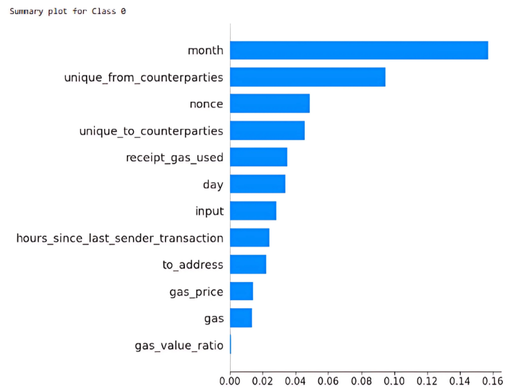
Figure 12. Global interpretation for Class 0.
