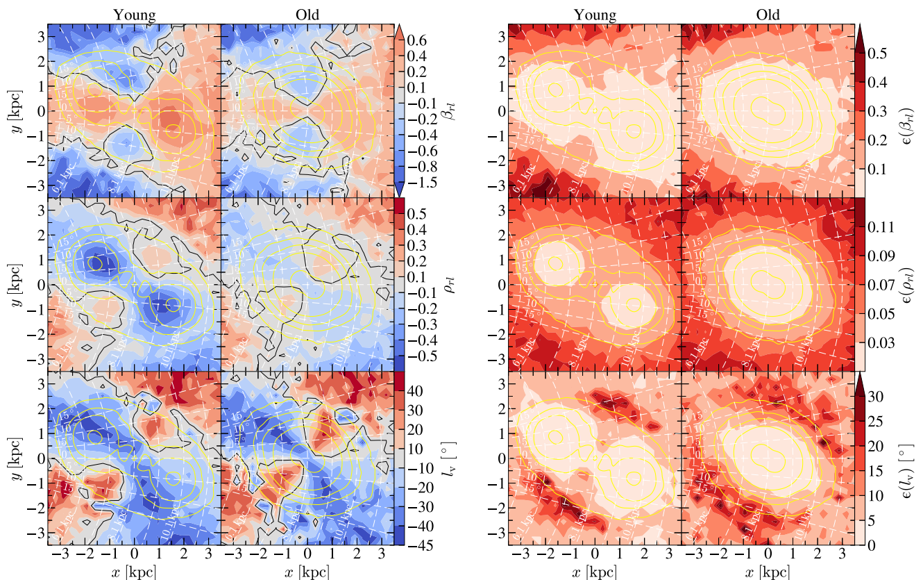
Figure 9. Same as Fig. 7, but now showing, from top to bottom, anisotropy ( \beta_{rI} ), correlation ( \rho_{rI} ), and the vertex deviation, l_v .
