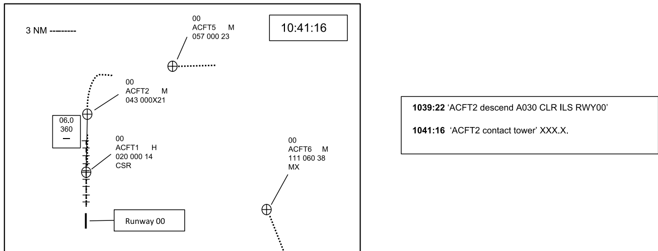
Fig. 4 Spacing ACFT 1 and 2 when ACFT2 turned onto final when instructed to contact the TWR CTR with transcript extract
