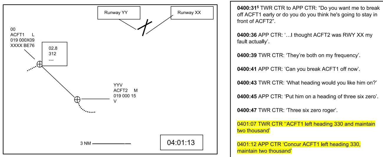
Fig. 7 Position of ACFT1 and ACFT2 when the minimum required separation of 3 NM was infringed and transcript extract
