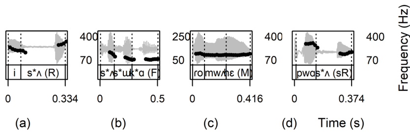
FIG. 1. Sample f_0 contours for (a) a rise (R), [i s*Λ] to be + INT, (b) a fall (F), [s*Λulɰk*α] PAST + INT, (c) a mid-tone (M) [romwΛhε], by what-do -INT and (d) a short rise (sR) [pwas*Λ], see + PAST + INT. Figure created using "praatpicture" version 1.5.0 (Puggaard-Rode, 2024).
