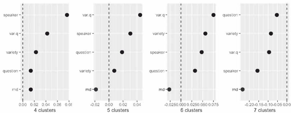
FIG. 3. Random forest outputs for four-, five-, six-, and seven-cluster rounds, abbreviations: variety \times question type interaction term (var.q), and random number (rnd).
