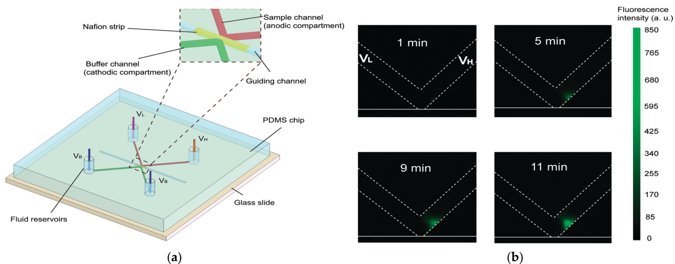
Figure 7. (a) Schematic description of a protein preconcentration chip integrating a Nafion strip demonstrating the buffer and the sample channels and the corresponding voltages ( V_B and V_L/V_H , respectively). The magnified view highlights the guiding channel designed for precise Nafion strip placement. (b) Fluorescence images showing preconcentration of 6 nM AF-BSA at 1, 5, 9, and 11 min after applying 10 V ( V_H = 15 V, V_L = 5 V); buffer reservoirs held at 0 V. Adopted from Reference [47].
