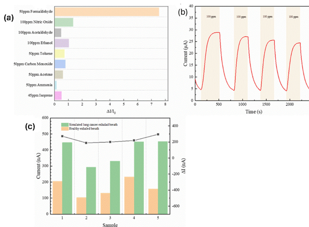
Figure 2. (a) Selectivity and (b) cycle stability of Nafion-based HCHO sensor. (c) Sensor's response to healthy individuals and simulated lung cancer patients. Adopted from reference [31].
