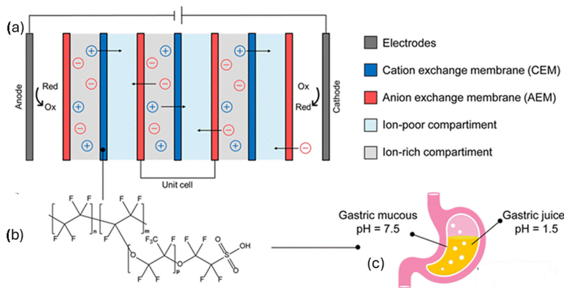
Figure 1. (a) Energy generation via reverse electrodialysis that relies on the use of Nafion (b) as the cation exchange membrane (CEM) and exploits the ionic gradient between the gastric mucus and the gastric juice (c). Adopted from reference [25].
