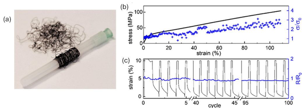
Figure 5. (a) Photograph of melt-spun PEDOT:Nafion fibers, wrapped around a 5 mm wide syringe cover. The evolution of electrical conductivity in PEDOT:Nafion fibers was evaluated during uniaxial stretching up to the point of mechanical failure (b) and during cyclic deformation within the elastic regime (c). Adopted from reference [41].
