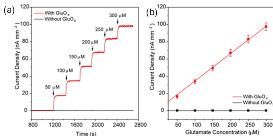
Figure 4. (a) Representative amperometric responses of the Nafion-coated NdNiO glutamate biosensor recorded at an applied potential of 0.6 V vs. Ag/AgCl in 0.01 M Phosphate-buffered saline (pH = 7.4), both in the presence and absence of Glutamate Oxidase (GluOx). (b) The corresponding calibration plots demonstrate a linear relationship between current density and glutamate concentration. Adopted from reference [40].
