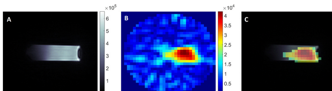
Figure 9. (A) ^1\text{H} MR image of an agar phantom containing Nafion based nanocarriers. (B) Corresponding ^{19}\text{F} MR image. (C) Overlay of the ^1\text{H} and ^{19}\text{F} MR images. Adopted from Reference [63].
