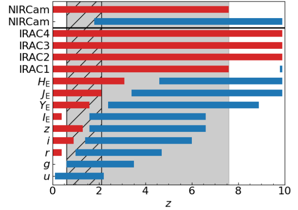
Fig. 1. Redshifts in which the different Euclid , IRAC, and ground-based filters trace the optical (red bars) or UV (blue bars) continuum. The grey shaded area indicates the redshift range in which we have at least four filters to derive the slopes necessary to select LRDs. The hatched area indicates the redshift range covered without IRAC. The first two bars, separated by a horizontal solid black line, indicate the redshift range in which at least two JWST NIRCcam broad-band filters trace the rest-frame optical or UV continuum.
