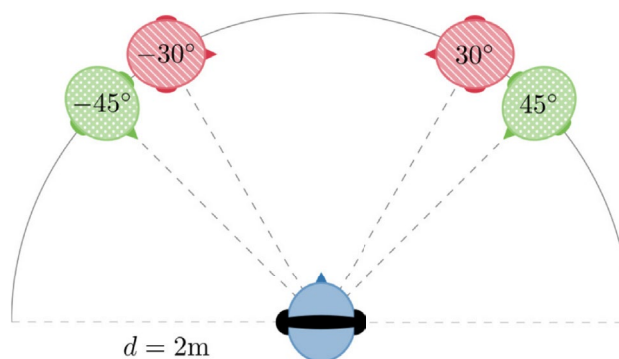
Fig. 1. Setup in Experiment 1. Target sources (green dashed circles) were placed virtually at \pm 45^\circ , noise sources (red solid circles) at \pm 30^\circ on the horizontal plane at a distance of d = 2\text{ m} from the receiver (blue circle) and played back via headphones.
