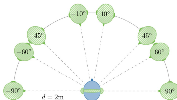
Fig. 3. Setup in Experiment 2. Target sequences (green) were reproduced spatially or monotic via headphones. Spatial target sources were placed virtually at \pm 10^\circ , \pm 45^\circ , \pm 60^\circ , \pm 90^\circ on the horizontal plane at a distance of d = 2 m from the receiver (blue).
