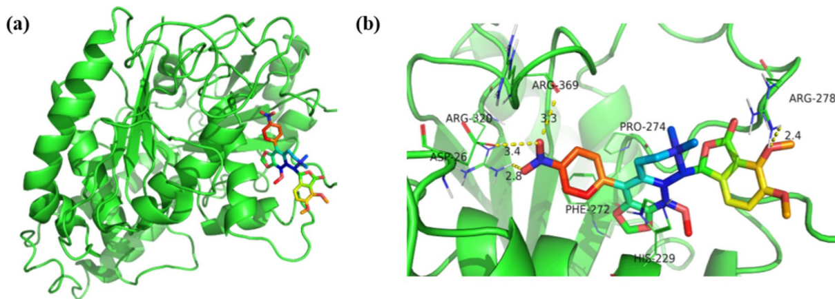
Fig. 3. Three dimensional docked poses of (a) [p\text{-NO}_2\text{-Nos}] I-tubulin interactions (b) Zoomed-in view of the docked complex.
