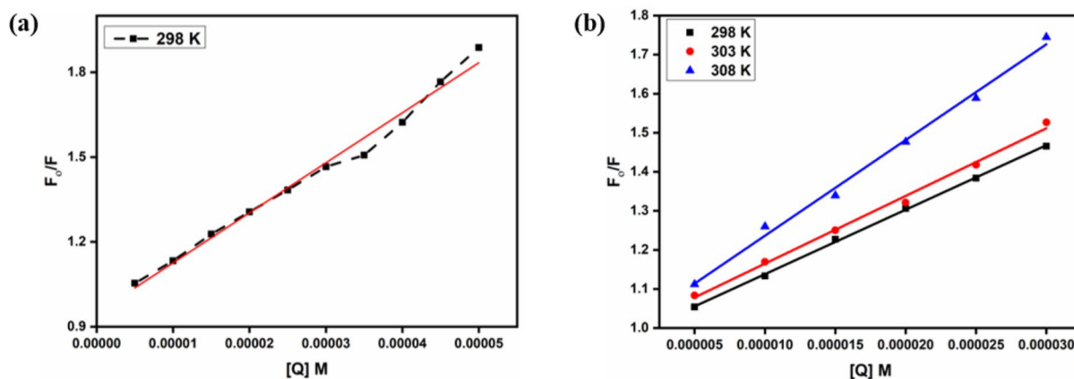
Fig. 7. Stern Volmer plot of Hb against different concentrations of (a) [p\text{-NO}_2\text{-Nos}]I at 298 K; (b) [p\text{-NO}_2\text{-Nos}]I (0 to 30 \mu\text{M} ) at 298 K, 303 K and 308 K.
