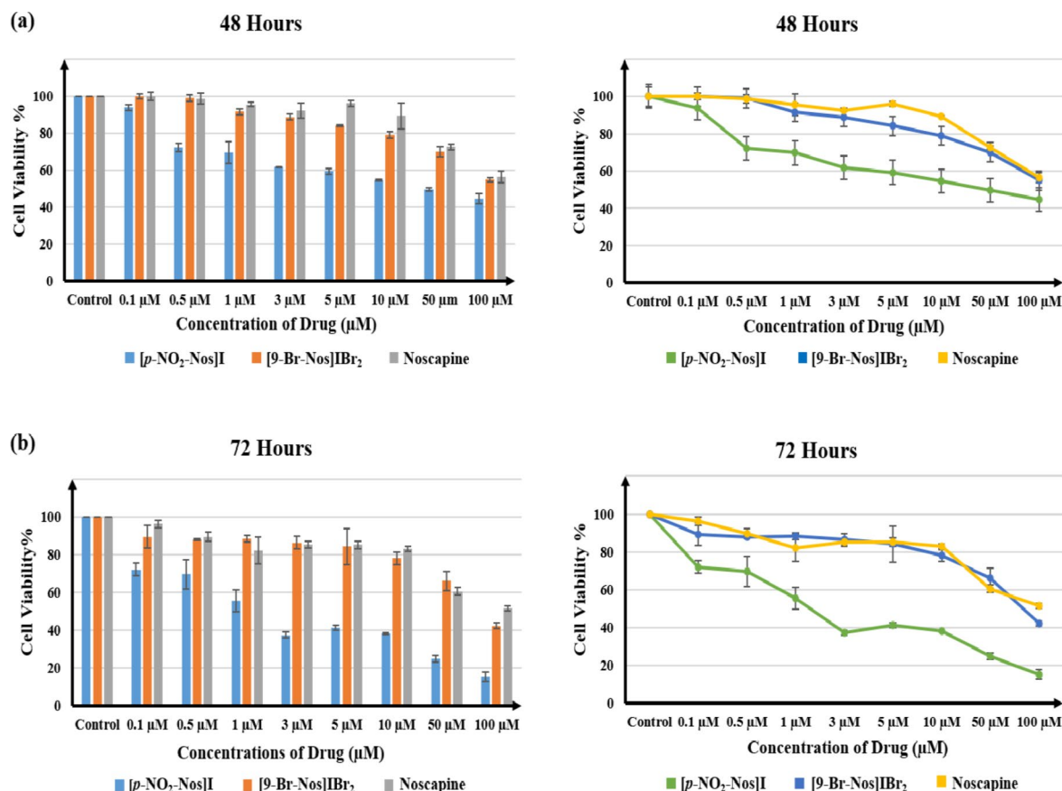
Fig. 10. Cytotoxicity profile of [p\text{-NO}_2\text{-Nos}]I , [9\text{-Br-Nos}]IBr_2 and Noscaphine at (a) 48 h, and (b) 72 h.
