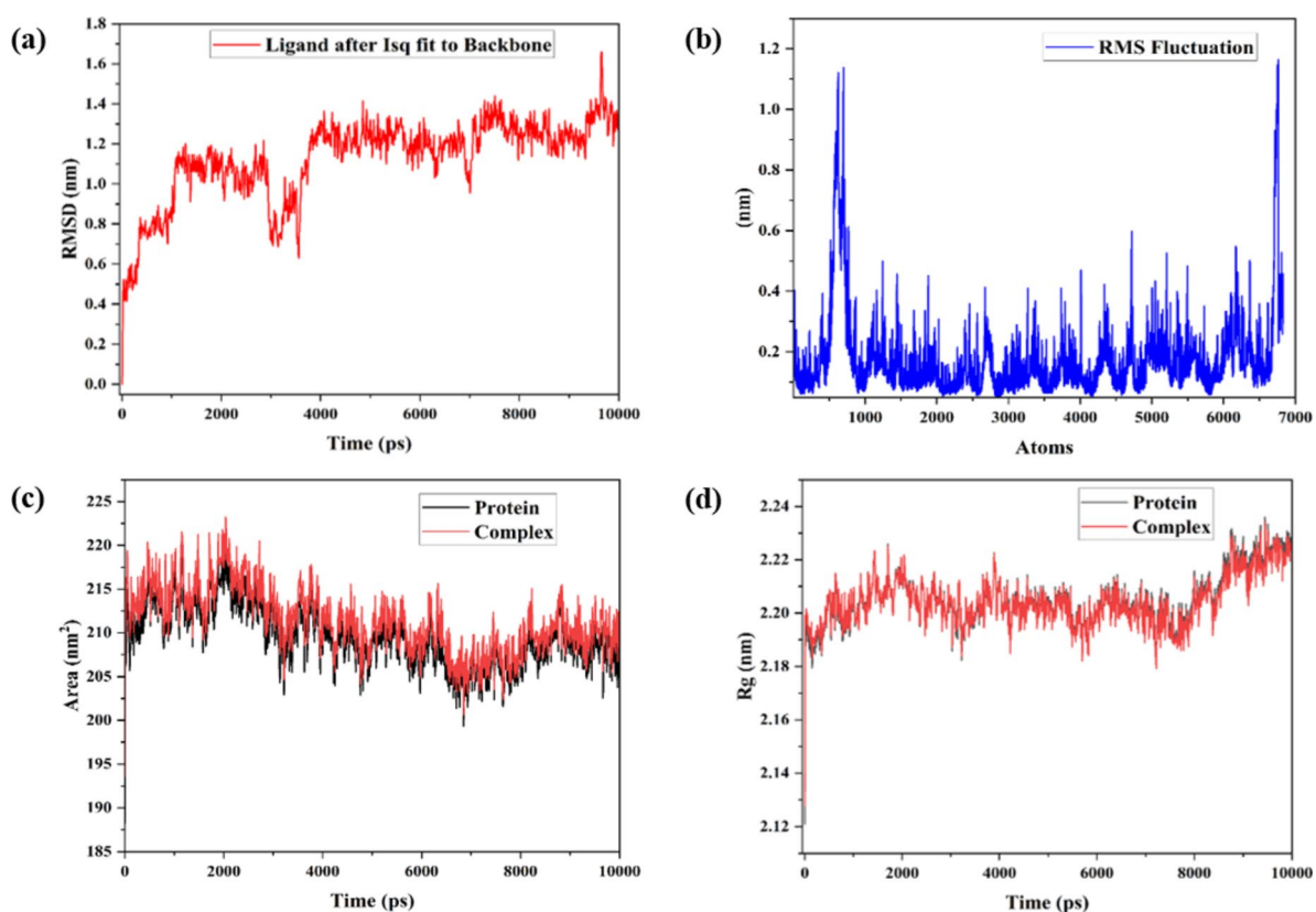
Fig. 4. MD simulation results of [p\text{-NO}_2\text{-Nos}] I-tubulin complex depicting (a) Root mean square deviation (RMSD); (b) Root mean square fluctuation (RMSF); (c) Solvent accessible area analysis (SASA); and (d) Radius of gyration.
