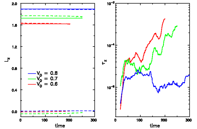
Figure 8. The dashed lines in the left panel indicate the separate angular momenta of the disks and halos, while the solid lines are their sum, demonstrating that this global integral is well conserved. The right panel gives the rates at which angular momentum is taken from the disk component and added to the halo.
