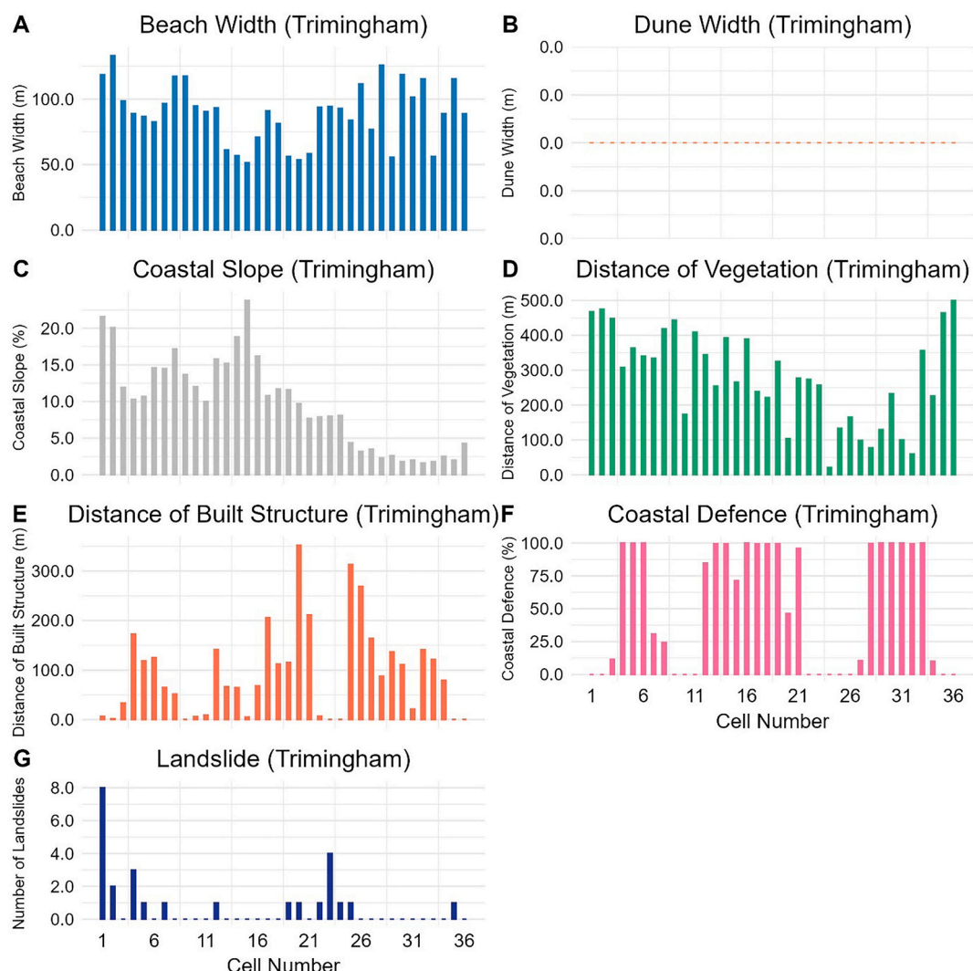
Fig. 8. Physical parameter measurement for Trimingham, where A) Beach width, B) Dune width, C) Coastal slope, D) Vegetation cover behind back beach, E) Built structure behind back beach, F) Coastal defence, and G) Coastal landslide.
