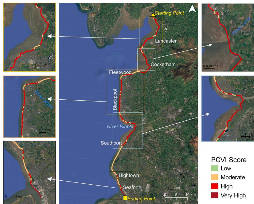
Fig. 13. PCVI Vulnerability map for Lancashire. It covers the coastline of the following districts (north to south): Lancaster, Wyre, Blackpool, Fylde, West Lancashire, and Sefton in Lancashire County.
