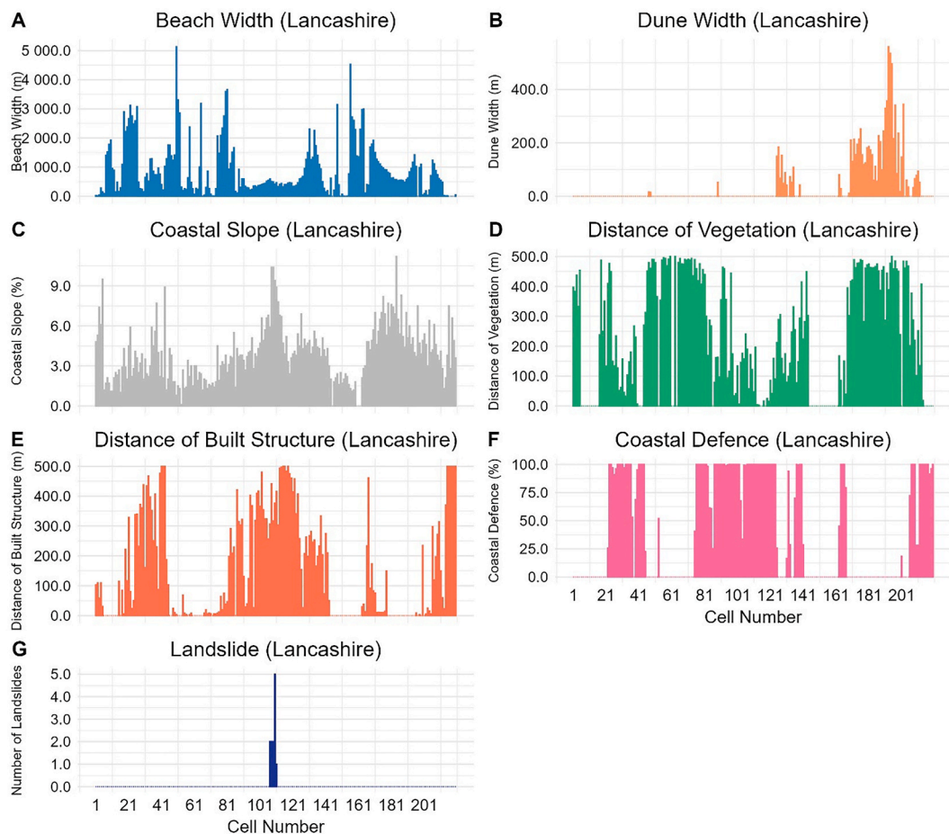
Fig. 12. Physical parameter measurement for Lancashire, where A) Beach width, B) Dune width, C) Coastal slope, D) Vegetation cover behind back beach, E) Built structure behind back beach, F) Coastal defence, and G) Coastal landslide.
