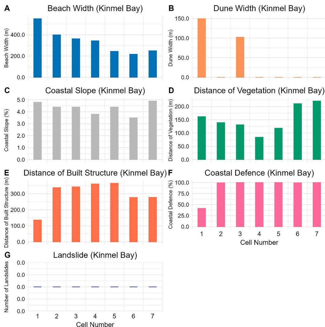
Fig. 14. Physical parameter measurement for Kinmel Bay, where A) Beach width, B) Dune width, C) Coastal slope, D) Vegetation cover behind back beach, E) Built structure behind back beach, F) Coastal defence, and G) Coastal landslide.
