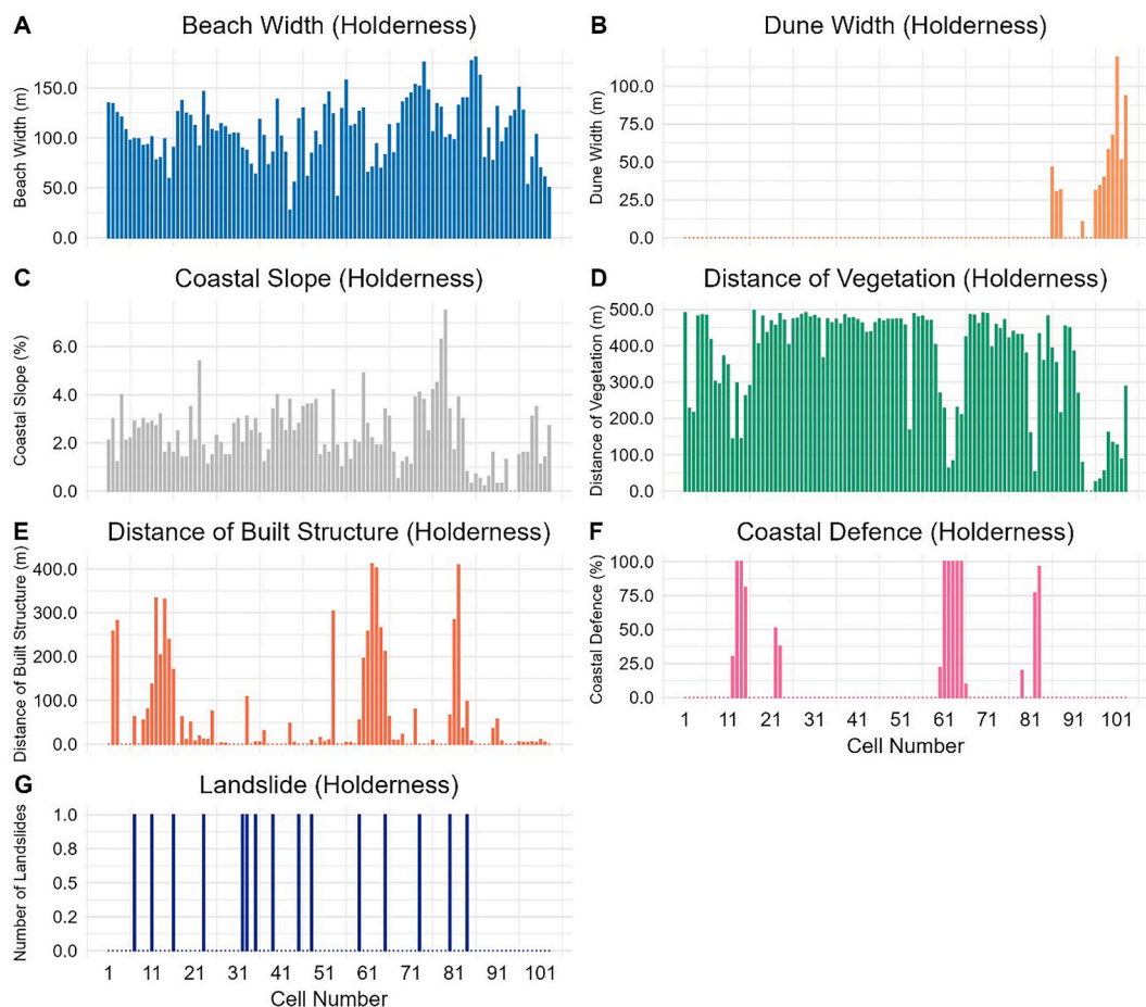
Fig. 6. Physical parameter measurement for Holderness, where A) Beach width, B) Dune width, C) Coastal slope, D) Vegetation cover behind back beach, E) Built structure behind back beach, F) Coastal defence, and G) Coastal landslide.
