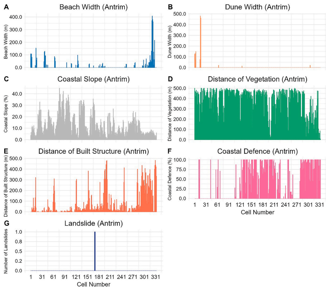
Fig. 20. Physical parameter measurement for Antrim, where A) Beach width, B) Dune width, C) Coastal slope, D) Vegetation cover behind back beach, E) Built structure behind back beach, F) Coastal defence, and G) Coastal landslide.
