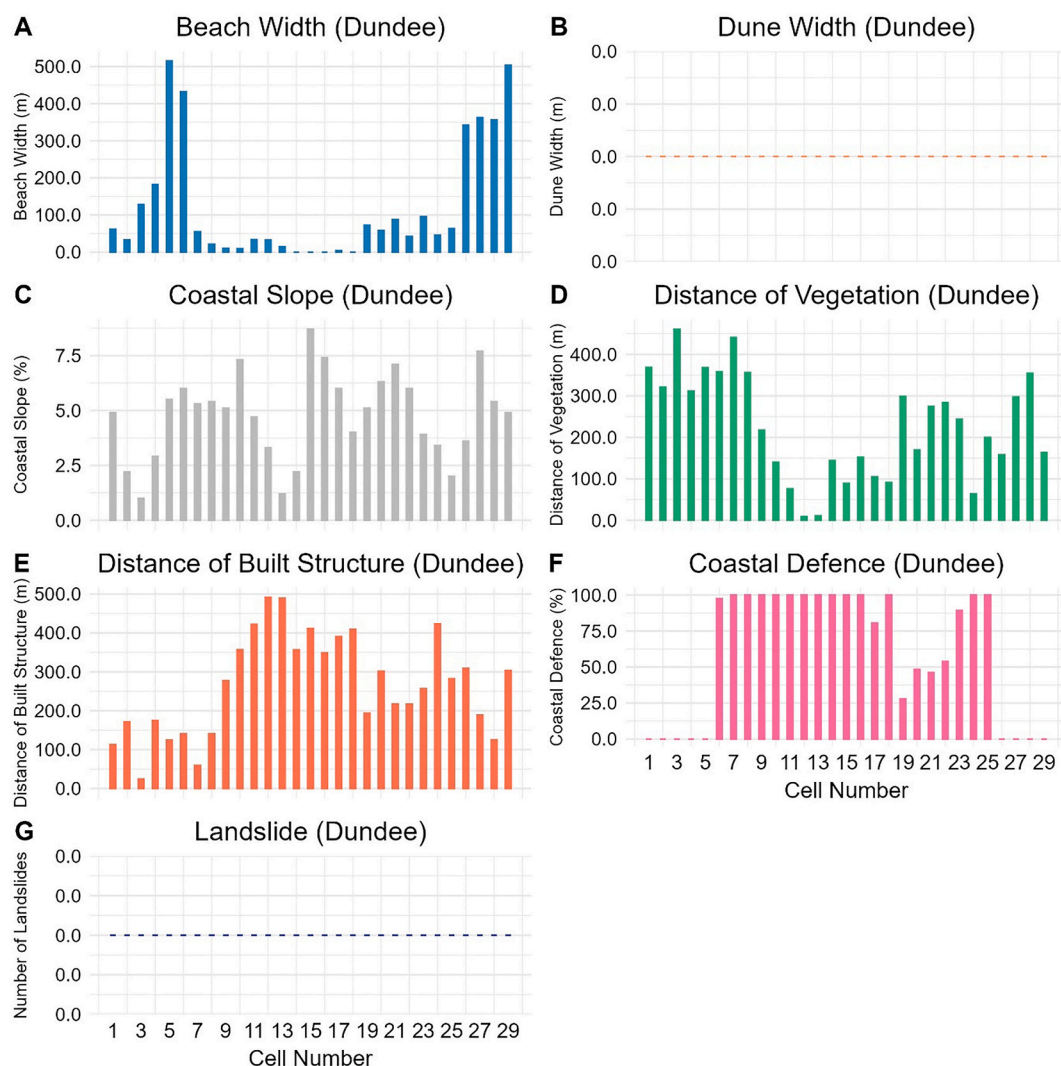
Fig. 16. Physical parameter measurement for Dundee, where A) Beach width, B) Dune width, C) Coastal slope, D) Vegetation cover behind back beach, E) Built structure behind back beach, F) Coastal defence, and G) Coastal landslide.
