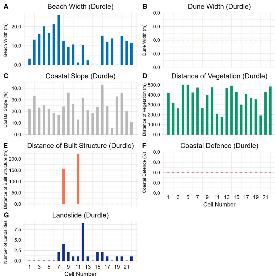
Fig. 10. Physical parameter measurement for Durdle, where A) Beach width, B) Dune width, C) Coastal slope, D) Vegetation cover behind back beach, E) Built structure behind back beach, F) Coastal defence, and G) Coastal landslide.
