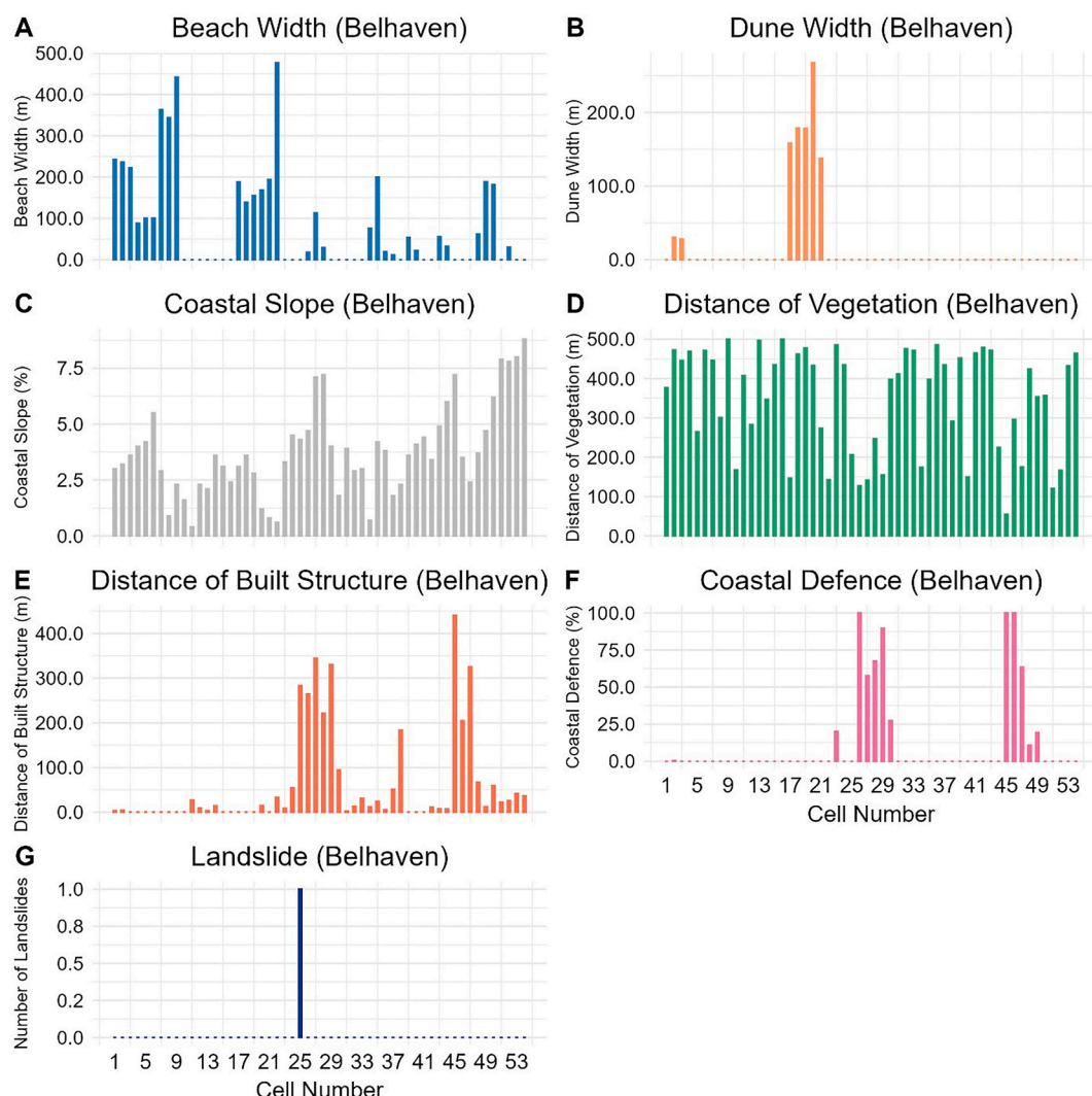
Fig. 18. Physical parameter measurement for Belhaven, where A) Beach width, B) Dune width, C) Coastal slope, D) Vegetation cover behind back beach, E) Built structure behind back beach, F) Coastal defence, and G) Coastal landslide.
