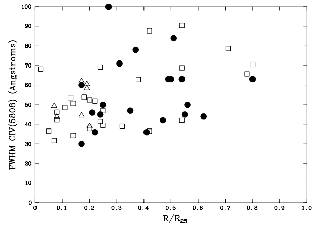
Figure 8. FWHM CIV\lambda 5808 increases with r/R_{25} for WC4-6 stars in NGC 7793 and M33. NGC 7793 data (circles) are plotted with unpublished WHT/WYFFOS (empty squares) and CFHT/MOS data (empty triangles) for M33 (Abbott et al. 2004).
