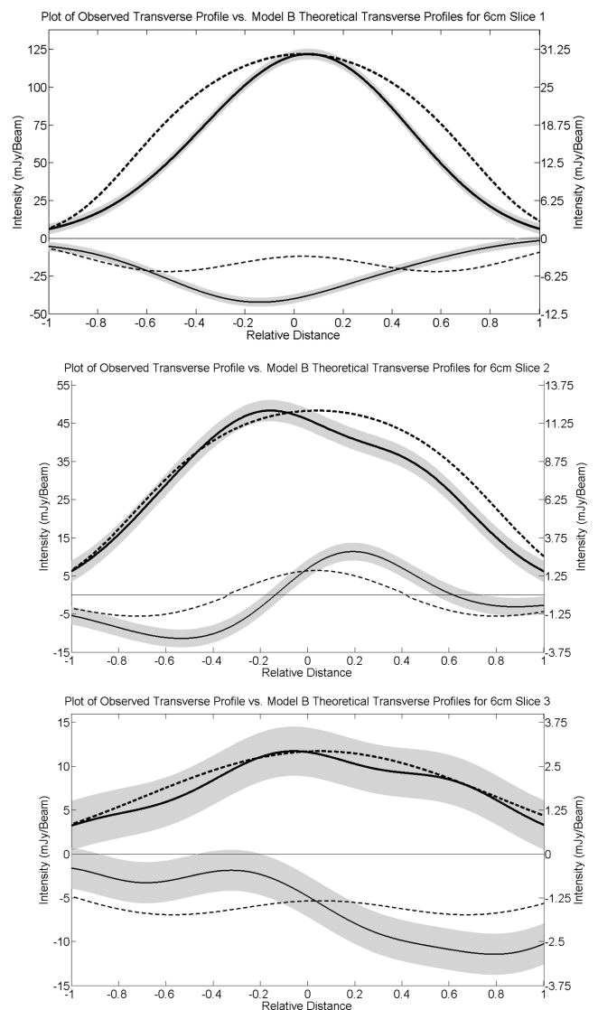
Figure 7. Plots of observed and best-fitting model I and Q profiles for 6-cm slices 1, 2 and 3 obtained for Model B of Laing (1981). The observed profiles are shown by the solid lines and the best-fitting profiles by the dashed line; the grey shaded areas surrounding the observed profiles correspond to the range of the 1\sigma uncertainties for Q and the 3\sigma uncertainties for I . The scale for the I profile is given along the left-hand vertical axis and the scale for the Q profile along the right-hand vertical axis. The beam is 1.8 mas along the slice and 2.4 mas transverse to the slice.
