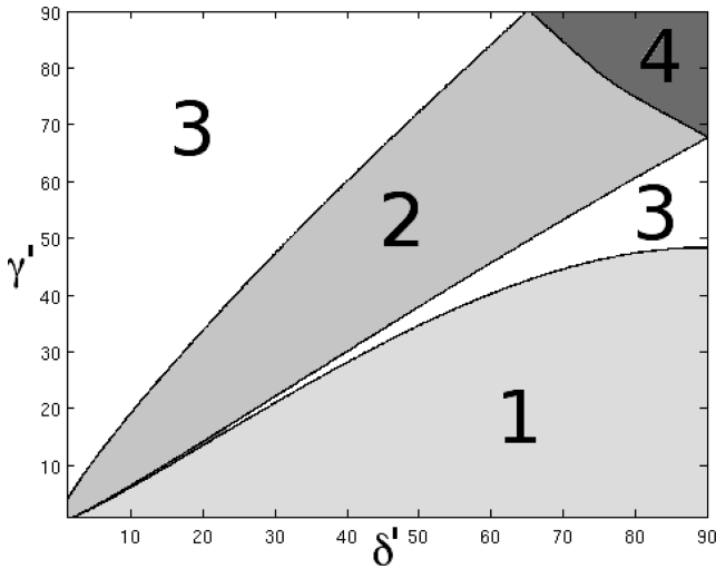
Figure 9. Magnetic field configuration map analogous to Fig. 2 for \alpha = 0.5 after convolution with a Gaussian beam with FWHM one quarter the size of the profile to mimic the effects of finite resolution. The region numbers correspond to the configuration types listed in Section 3.
