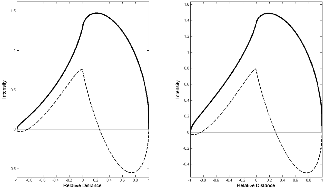
Figure 8. Theoretical profiles generated numerically for \gamma' = 60^\circ , \delta' = 40^\circ and f = 0 . The left-hand and right-hand profiles were determined for \alpha = 1.0 and 0.5 , respectively. The magnetic field orientation is perpendicular to the polarization orientation.
