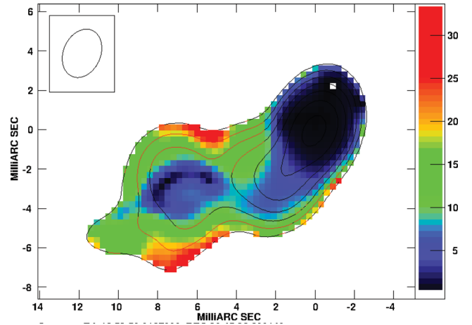
Figure 10. 6-cm total intensity contours given in Fig. 3 superposed with a colour image of the distribution of the degree of polarization. The increase in the degree of polarization towards the edges of the jet, also reported by Pushkarev et al. (2005), is clearly visible. The locations of the highest degrees of polarization do not coincide with those expected for curvature-induced polarization.
