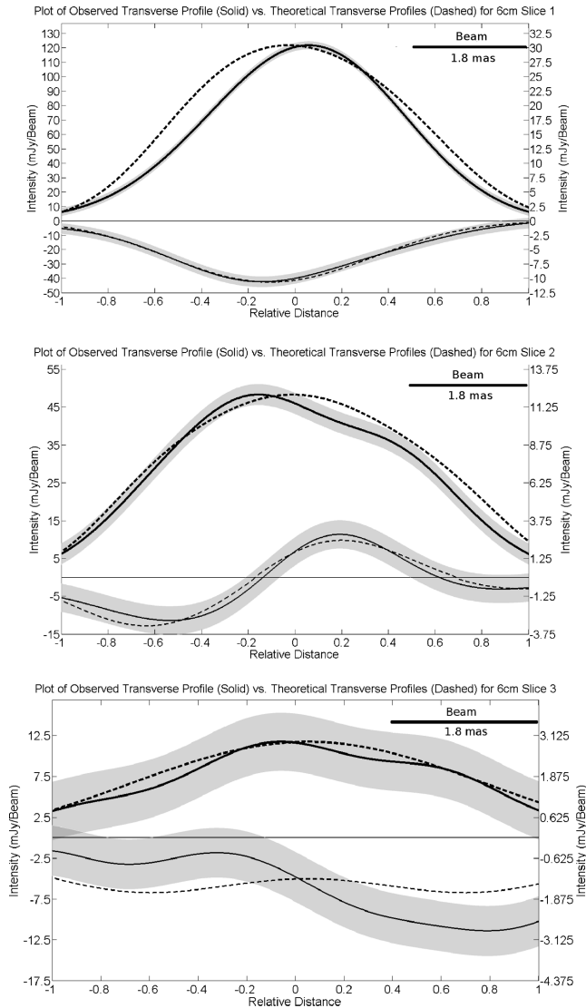
Figure 5. Plots of observed and best-fitting model I and Q profiles for slices 1, 2 and 3 (top to bottom) of the 6-cm Mrk 501 map (see Fig. 3). The observed profiles are shown by the solid lines and the best-fitting profiles by the dashed line; the grey shaded areas surrounding the observed profiles correspond to the range of the 1\sigma uncertainties for Q and the 3\sigma uncertainties for I . The scale for the I profile is given along the left-hand vertical axis and the scale for the Q profile along the right-hand vertical axis. The beam is 1.8 mas along the slice and 2.4 mas transverse to the slice.
