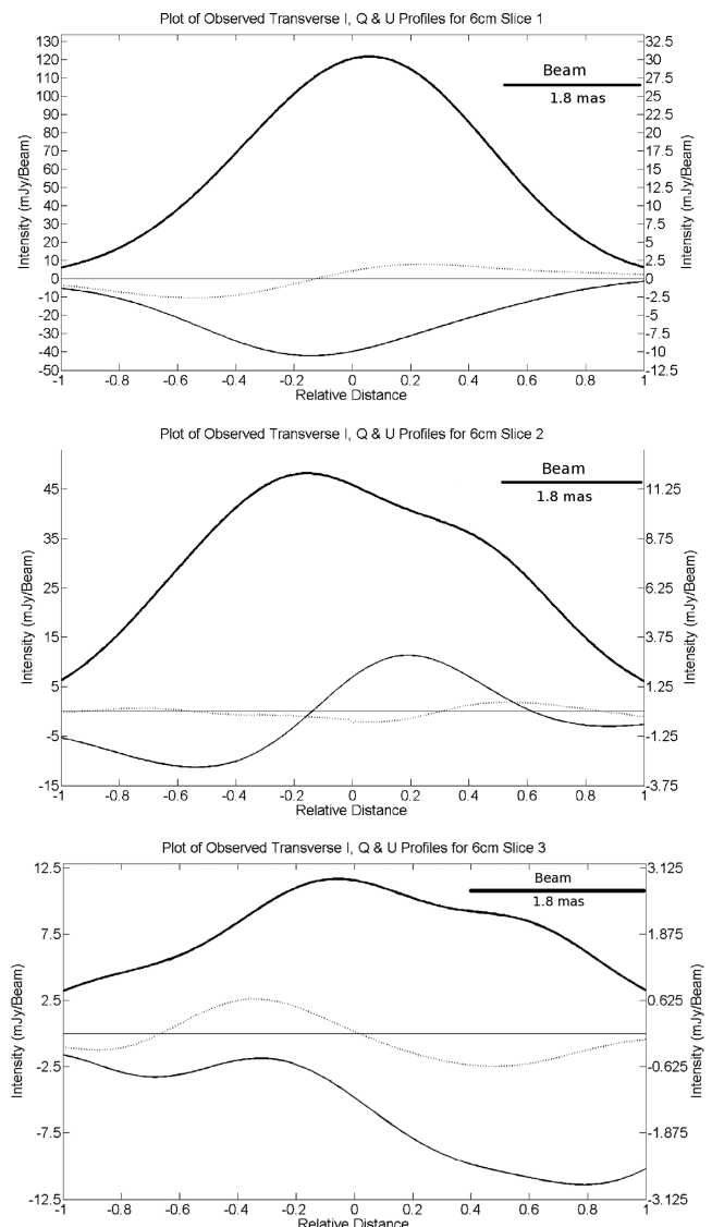
Figure 4. Observed I (solid line), Q (dashed line) and U (dotted line) profiles for slices 1, 2 and 3 (top to bottom) of the 6-cm Mrk 501 map (see Fig. 3). The scale for the I profile is given along the left-hand vertical axis and the scale for the Q and U profiles along the right-hand vertical axis. The beam is 1.8 mas along the slice and 2.4 mas transverse to the slice.
