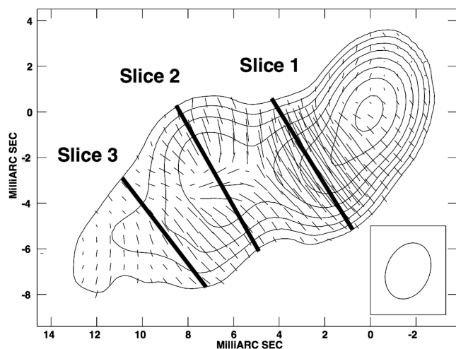
Figure 3. 6-cm polarization map of Mrk 501 for 1997 February (Pushkarev et al. 2005). The polarization sticks are proportional to the polarized intensity. The three lines across the jet show the transverse slices that were analysed. The peak intensity is 0.52 \text{ Jy beam}^{-1} , and the contour levels are 0.60, 1.25, 2.5, 5.0, 10.0, 20.0, 40.0 and 80.0 per cent of the peak.
