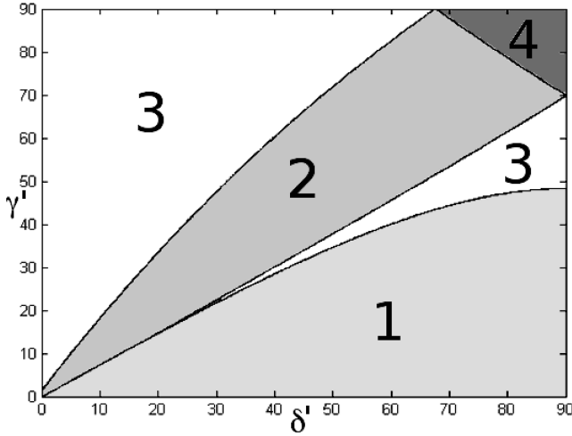
Figure 2. Effect of finite resolution on the observed magnetic field configurations. Convolution was performed using a Gaussian beam with a FWHM one quarter the size of the intrinsic jet width. The region numbers correspond to the configuration types listed in Section 3.
