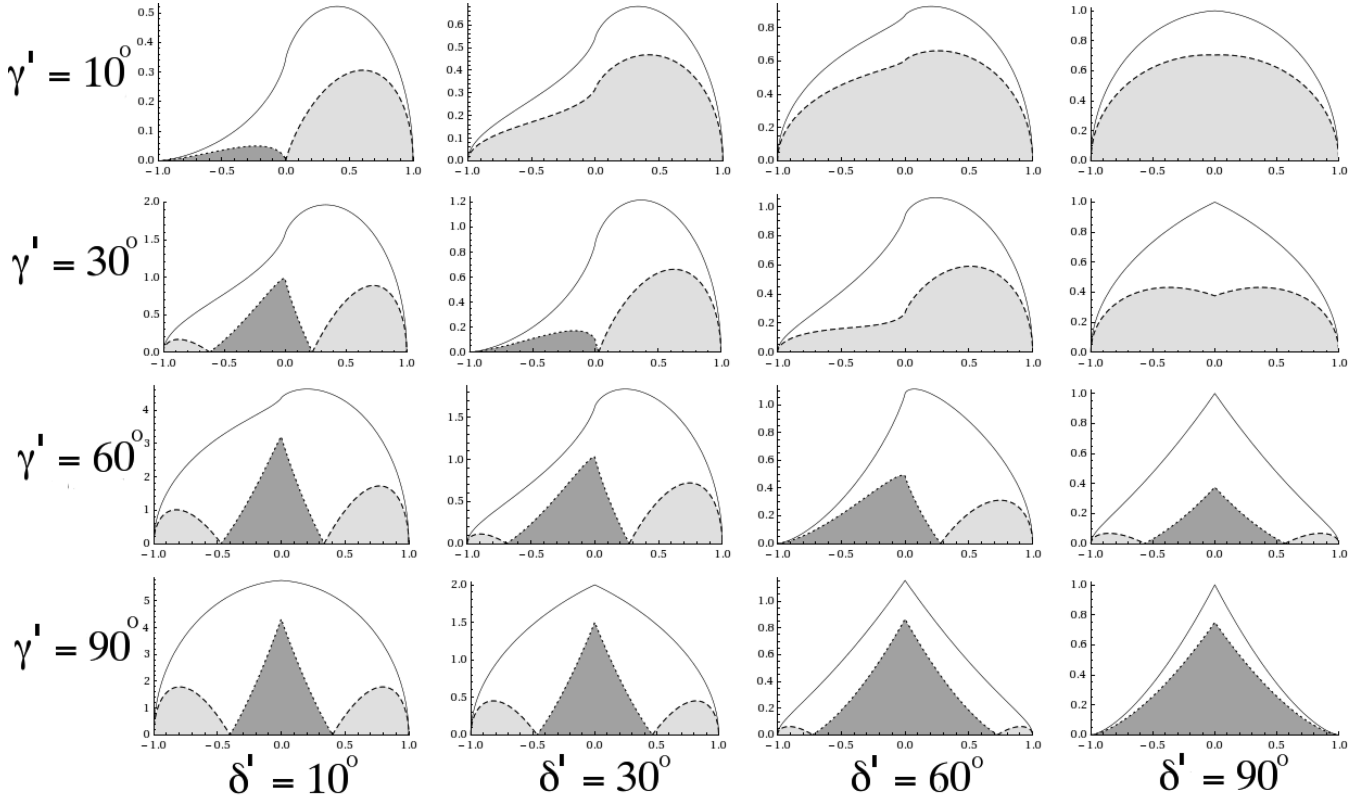
Figure 1. Transverse structure produced by the model considered, for various viewing angles, \delta' , and helix pitch angles, \gamma' . The solid lines correspond to the total intensity, dark grey regions to longitudinal polarization (EVPAs aligned with the jet) and light grey regions to transverse polarization (EVPAs orthogonal to the jet).
