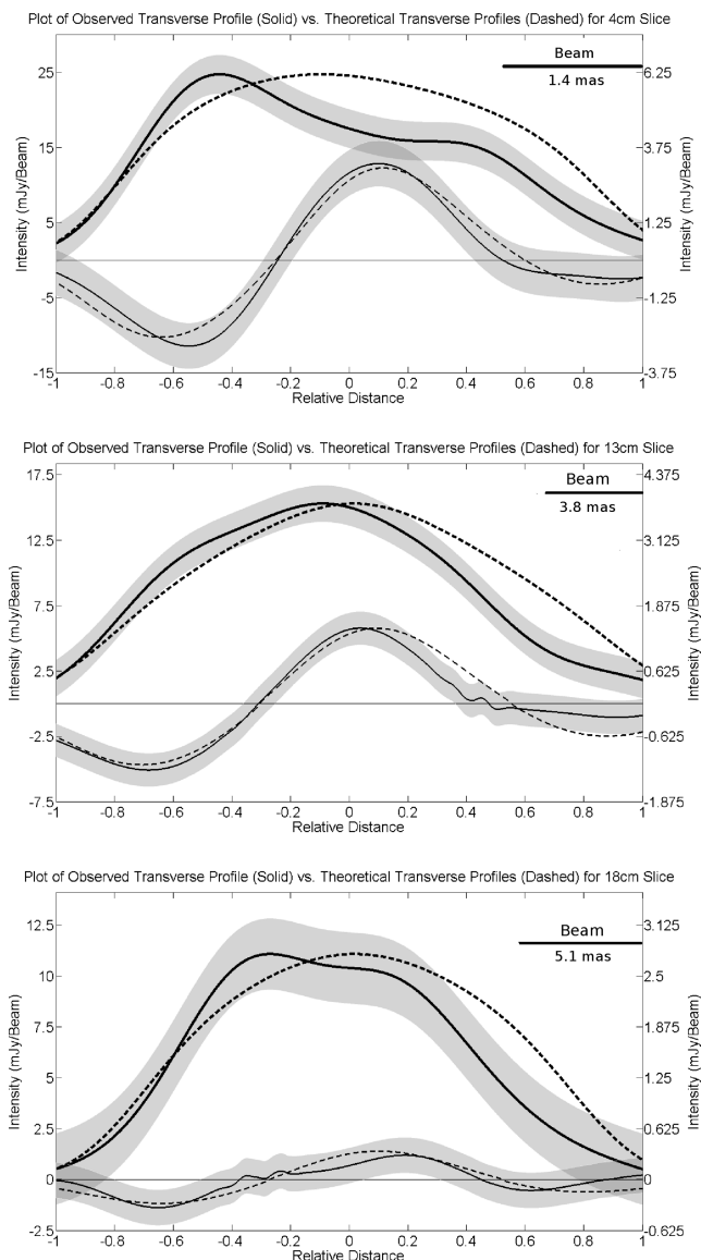
Figure 6. Plots of observed and best-fitting model I and Q profiles for 4-cm (top), 13-cm (middle) and 18-cm (bottom) slices taken in the same region as slice 2 (see Fig. 3). The observed profiles are solid and the best-fitting profiles dashed; the grey shaded areas surrounding the observed profiles correspond to the range of the 1\sigma uncertainties for Q and the 3\sigma uncertainties for I . The scale for the I profile is given along the left-hand vertical axis and the scale for the Q profile along the right-hand vertical axis. The beam sizes along and transverse to the slice are 1.4 and 1.6 mas (4 cm), 3.8 and 2.8 mas (13 cm), and 5.1 and 3.8 mas (18 cm).
