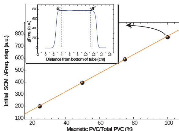
Fig. 2. Testing of the SCM output reading as a function of a suspension's magnetic pigment concentration. Each data point was found using the mean of the initial step on newly produced (homogenous) dispersions and is shown at full magnetic PVC in the inset with the calculation taken between points a and a'.
