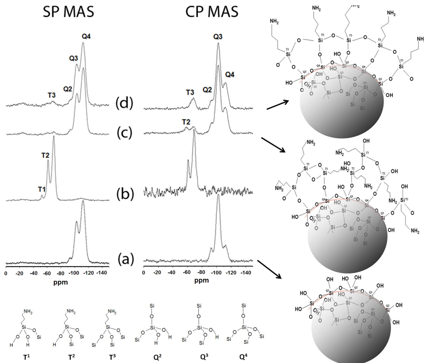
Figure 3 | ^{29}\text{Si} single pulse (SP) and ^{29}\text{Si} - ^1\text{H} cross polarization (CP) magic angle sample spinning (MAS) spectra of non-aminosilatised diamagnetic silica nanoparticles. (a); condensed/polymerised APTS (b); silica nanoparticles aminosilatised in water (c) and silica nanoparticles aminosilatised via TPPE (d).
