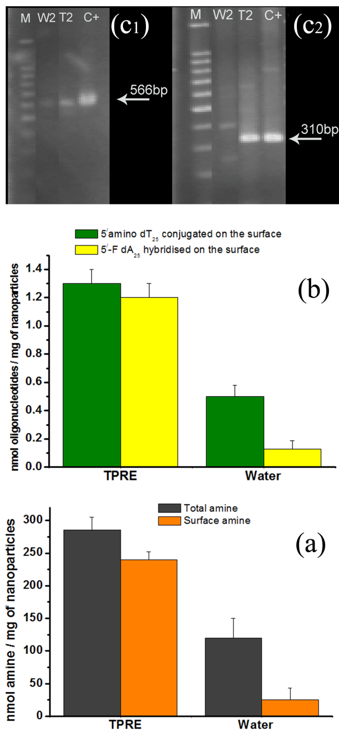
Figure 2 | Total and surface amine densities of nanoparticles aminosilanised via TPPE and in water. (a); 5'-NH 2 dC 6 dT 25 oligonucleotide grafted and hybridized 5'-FdA 25 complementary oligonucleotide (b); hybrid capture using bacterial genomic DNA. PCR amplification of 566 bp bacterial 16S rRNA gene fragment (c1) and 310 bp pfkB-thrS intergenic region from Salmonella enterica (c2). Abbreviations: M, 100 bp DNA molecular weight ladder (New England Biolabs Inc); W silica-magnetic nanoparticles aminosilanised in water and T aminosilanised silica-magnetite nanoparticles produced via TPPE; 1 and 2 correspond to 16S rRNA and Salmonella enterica DNA sequences, respectively; C+, positive PCR control.
