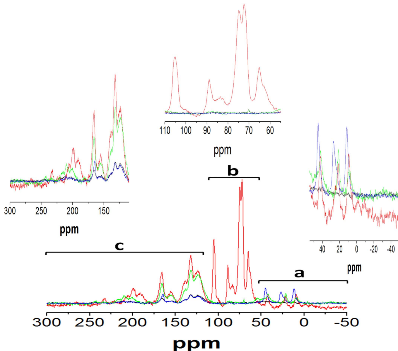
Figure 4 | ^{13}\text{C} - ^1\text{H} CPMAS NMR spectra of: non-aminosilanised silica nanoparticles (black); condensed/polymerised APTS (blue); unwashed TPRE aminosilanised silica nanoparticles (red); and washed TPRE aminosilanised nanoparticles (green).
