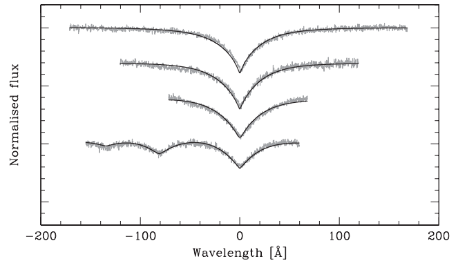
Figure 3. High-resolution spectra of WD1017–138 taken with the UVES spectrograph on the VLT. White dwarf models fitted to the Balmer lines of hydrogen ( H\beta , H\gamma , H\delta and H\epsilon and H8 and H9 , from top to bottom) give T_{\text{eff}} = 32600 K, \log g = 7.8 (cgs) for an inferred mass of 0.55 M_{\odot} , in good agreement with other determinations. The spectra also show that WD1017–138 is a DA hydrogen atmosphere white dwarf with no trace of helium in its spectrum.
