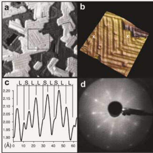
FIG. 2 (color). (a) 400 \times 400 \text{ Å} STM image of the fivefold surface of Al-Pd-Mn after deposition of 5.5 ML of Cu. (b) 100 \times 100 \text{ Å} detail from (a). (c) A profile between the points marked with a cross in (b); it demonstrates that the sequence of Cu rows is quasiperiodic with spacings given by LSLLSLSLL , where S = 4.5 \pm 0.2 \text{ Å} and L = 7.3 \pm 0.3 \text{ Å} . The ratio of these numbers equals the golden mean \tau within experimental error. (d) LEED pattern (beam energy 50 eV) corresponding to this phase. The relationships between spot positions are indicative of \tau scaling.
