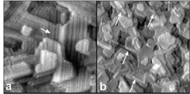
FIG. 3. (a) 350 \times 350 \text{ Å} STM image of the Al-Pd-Mn surface dosed with 8.7 ML of Cu. The correlation of the row structures across four atomic steps is indicated by the arrow. (b) 800 \times 800 \text{ Å} image of the surface after adsorption of 11.7 ML. The features highlighted by arrows are discussed in the text.
